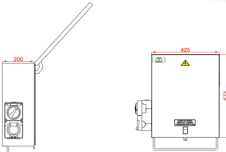
**Dimensions TPB-3PT5.532
