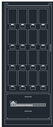
Part No -RMP-B Enclosure 800Wx2020Hx250D Ingress Protection: IP40 16 Single Phase 9 Three Phase
