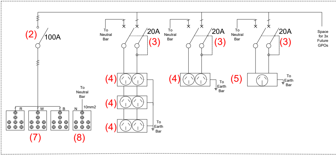
SLD
