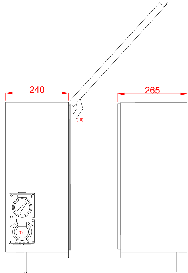
Profile View LHS Door Open Profile View RHS Door Closed
