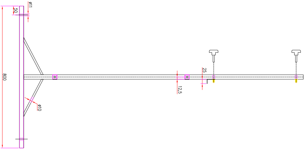
TPB Stand Profile
