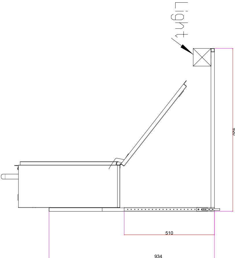
Profile View with DSD TPB
