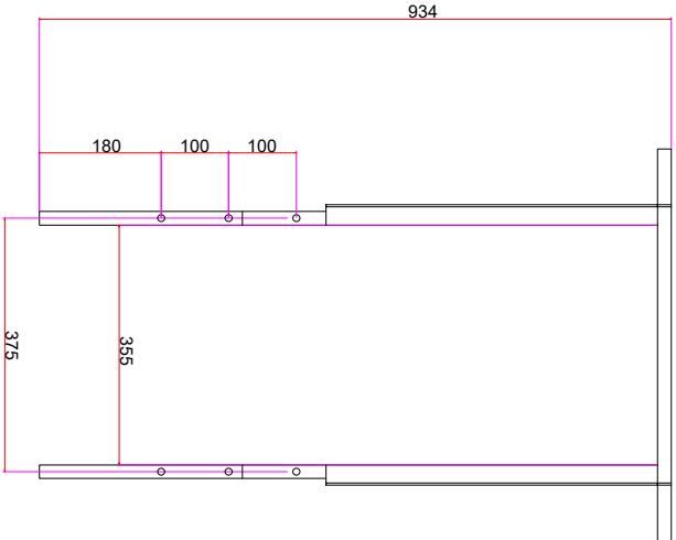
Front View View
